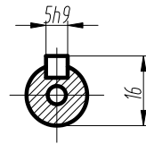
Standard output shaft
